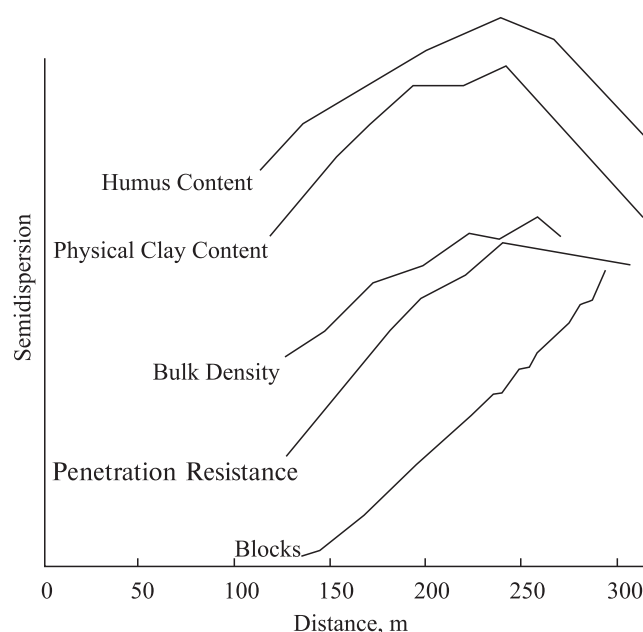
Fig. 1. Co-Variograms of Base and Functional Indicators For 0 to 10 cm Soil Layer of the Examined Field
